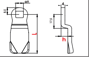
Paslanmaz Diller Stainless Steel Cams
